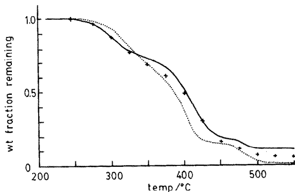
Fig. 3. TG curves of PVC/ \alpha MSAN (50:50) blends: —, immiscible blend; +, miscible blend; (· · · · ·), predicted by the additivity rule.
